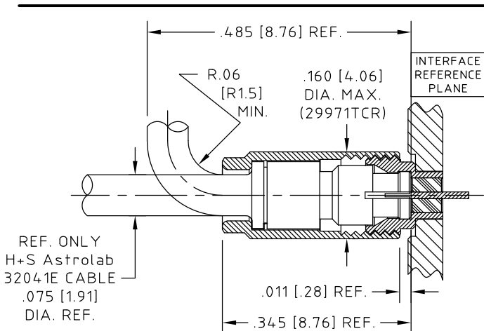
FIGURE 3 SCALE 4 : 1 SHOWN ABOVE IS TYPICAL APPLICATION UTILIZING AN H+S Astrolab SMPM-T FEMALE CONNECTOR (29971TCR SERIES) MATED AND LOCKED.
