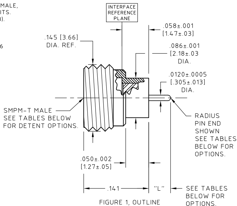
FIGURE 1, OUTLINE 29976H1-X-NNNS
